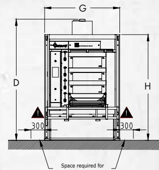
FRONT VIEW WITH INTEGRATED LIFTER
