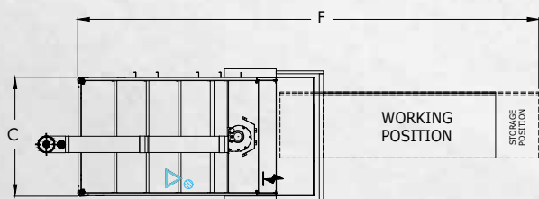
TOP VIEW WITH INTEGRATED LIFTER
